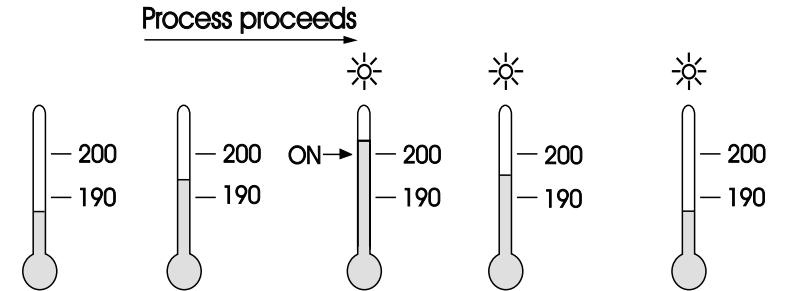
Figure 3.4 Latching Process Alarm
