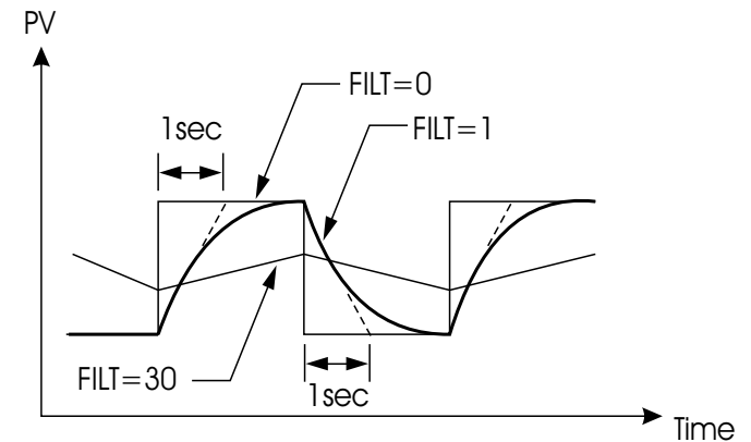
Figure 3-2 Filter Characteristics
