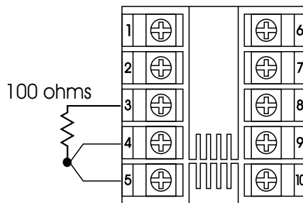
Figure 5-3 RTD Calibration
