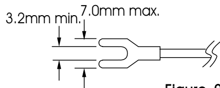
Figure 2-2 Lead Termination
