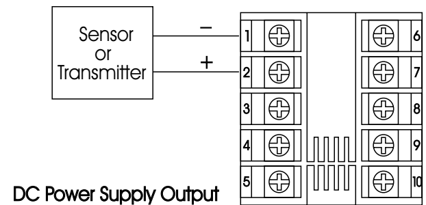
Figure 2-11 Output 2 Wiring
