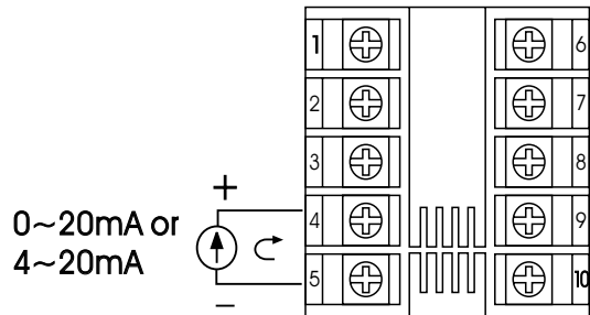
Figure 2.8 Linear Current Input Wiring *
