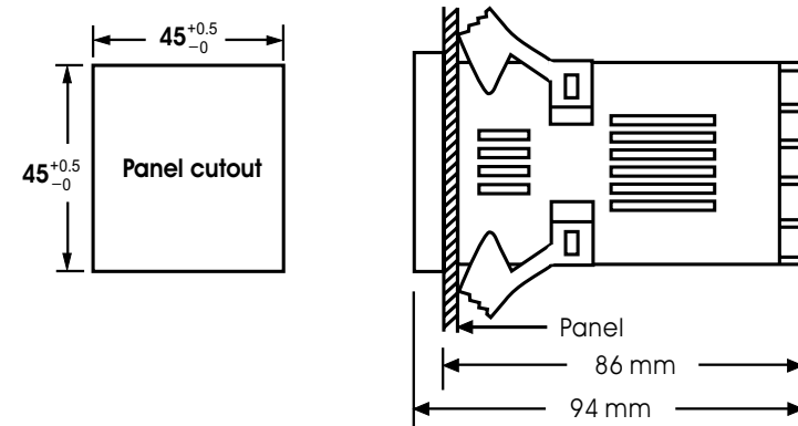
Figure 2-1 Mounting Diagram
